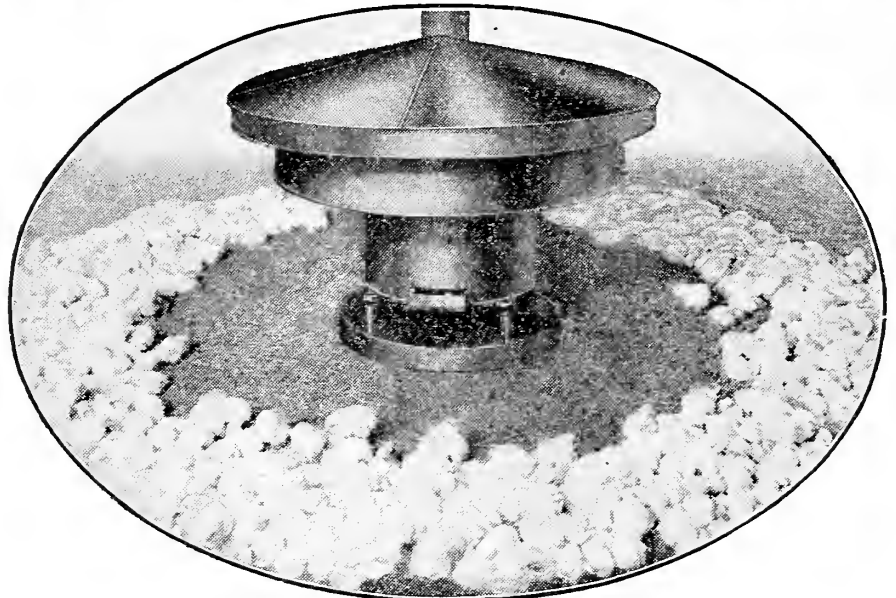
Simplex Brooder Stove
